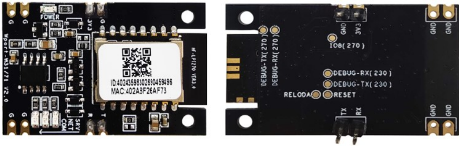
Figure 4. Wport-W71-AA-1(2M)外观图
