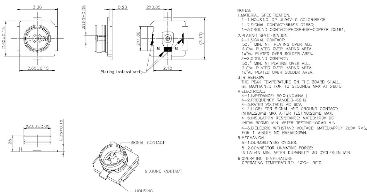
Figure 10. 1代 IPEX 焊盘尺寸
