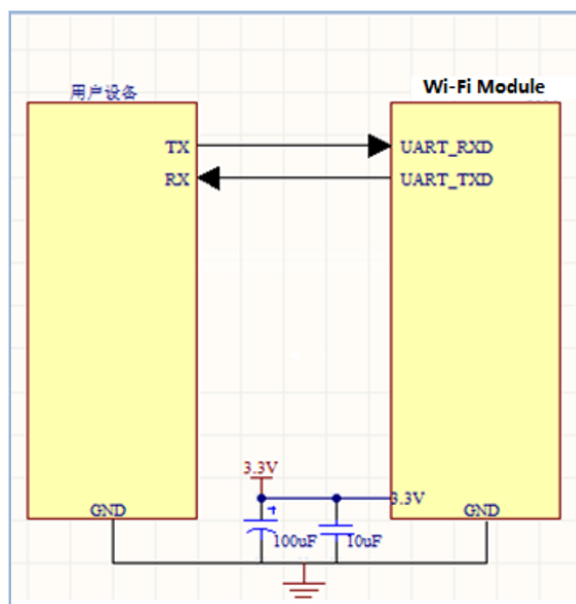
Figure 12. UART 应用硬件连接
