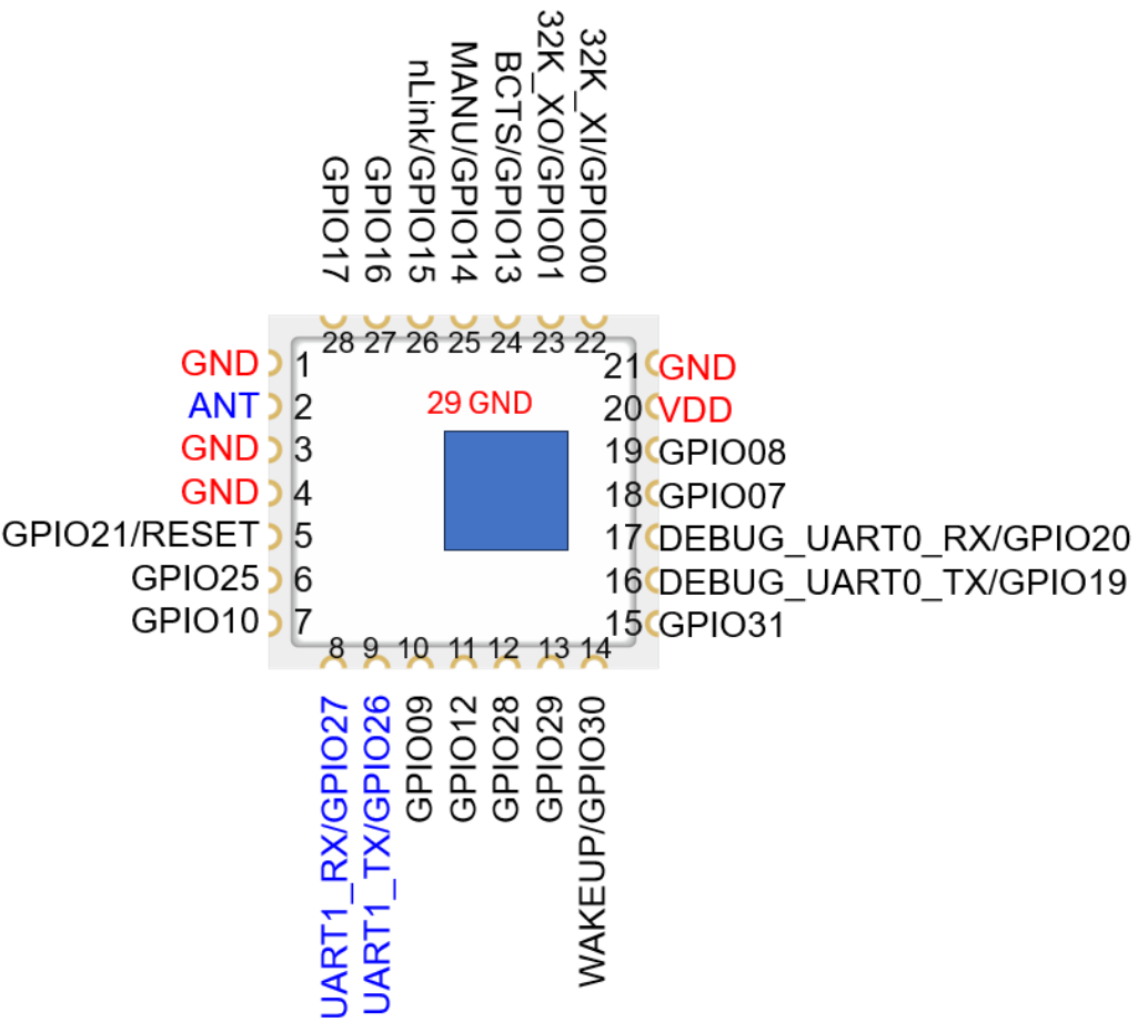
Figure 3. HF-BSL630-2 管脚定义
