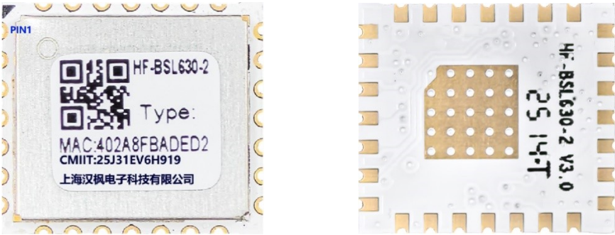
Figure 2. HF-BSL630-2 外观图
