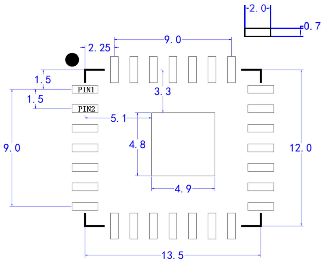
Figure 5. 封装尺寸
