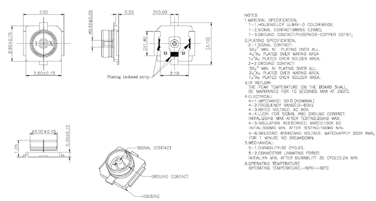
Figure 7. 1代 IPEX 焊盘尺寸
