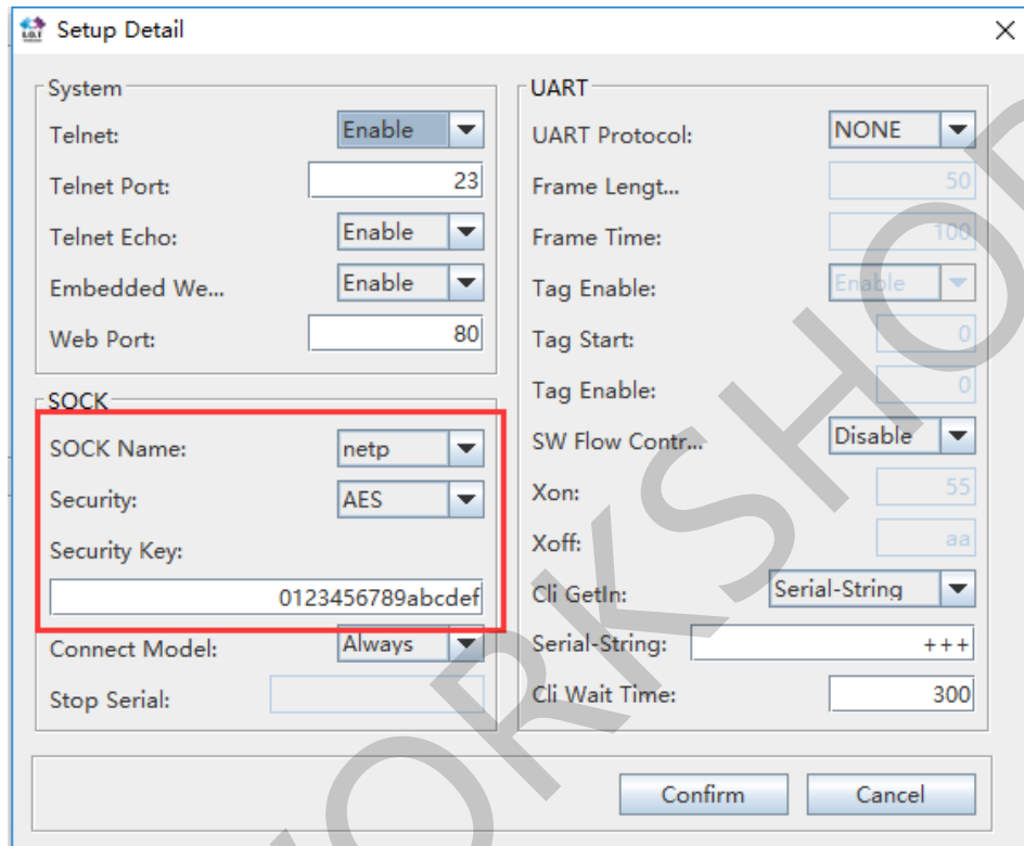
Figure 23. IOTManager 软件配置加密
