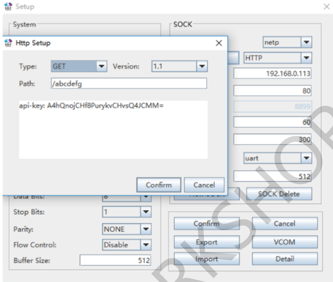
Figure 17. IOTManager 软件配置
