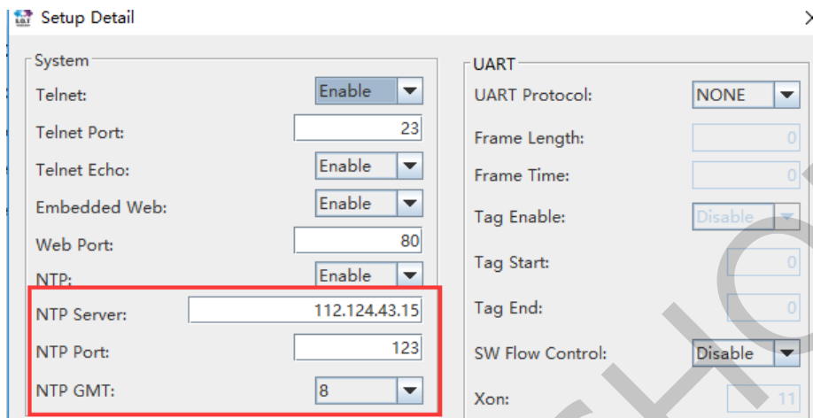
Figure 44. IOTManager NTP 相关设置
