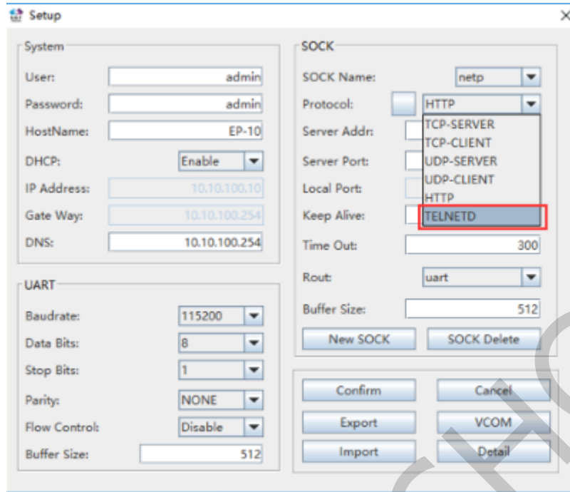
Figure 20. IOTManager 软件配置协议
