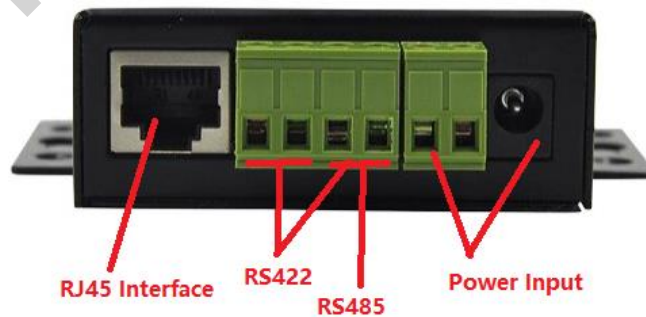
Figure 3. HF5111B 侧面图
