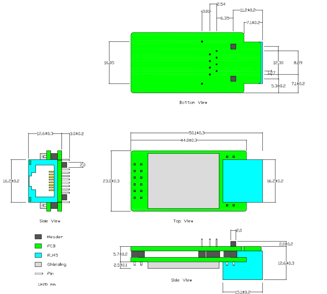
Figure 6. Eport Pro-EP20 机械尺寸
