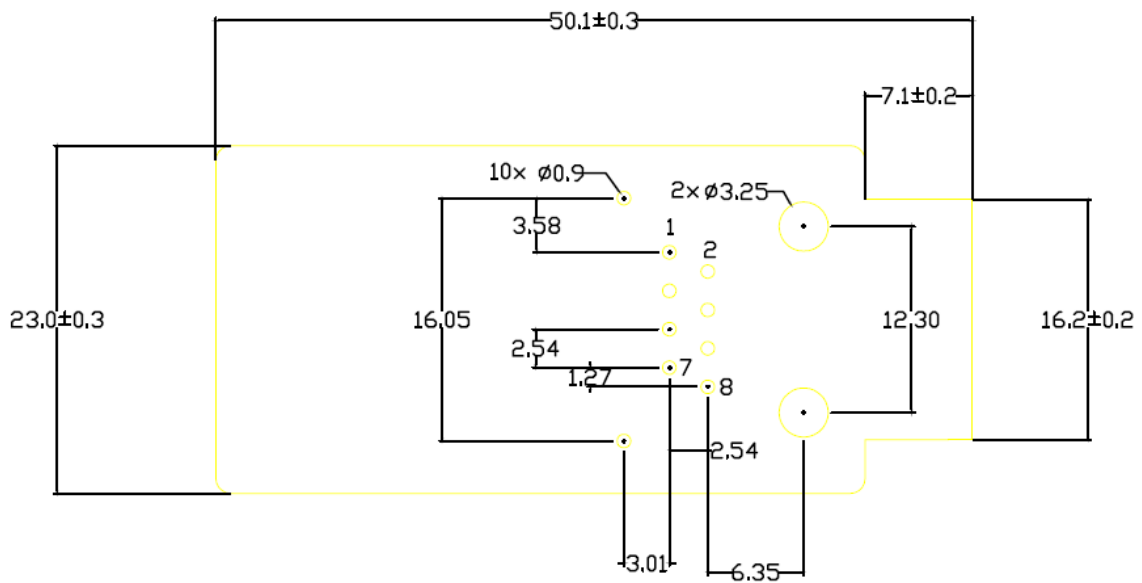
Figure 7. Eport Pro-EP20-PIN 推荐 PCB 封装
