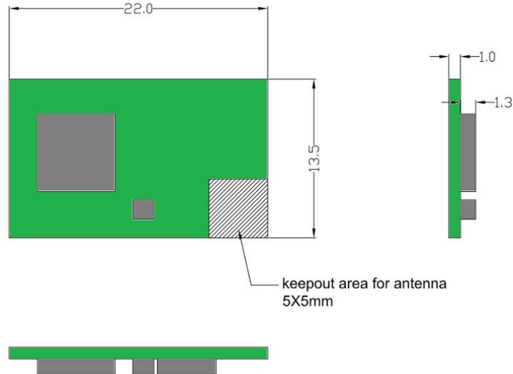
Figure 2. HF-LPT220 Mechanical Dimension
