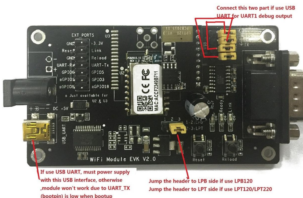
Figure 5. LPT120/LPT220 EVK
