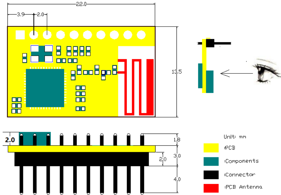
Figure 2. HF-LPT120 机械尺寸
