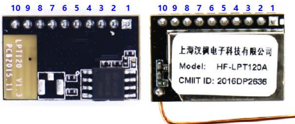
Figure 1. HF-LPT120 管脚定义
