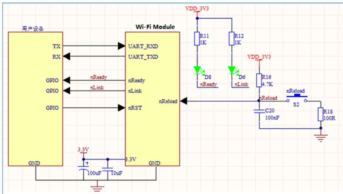
Figure 9. HF-LPT120UART 应用硬件连接
