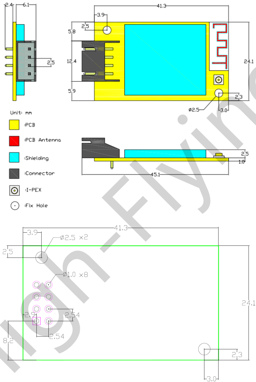
Figure 2. HF-LPB125 机械尺寸
