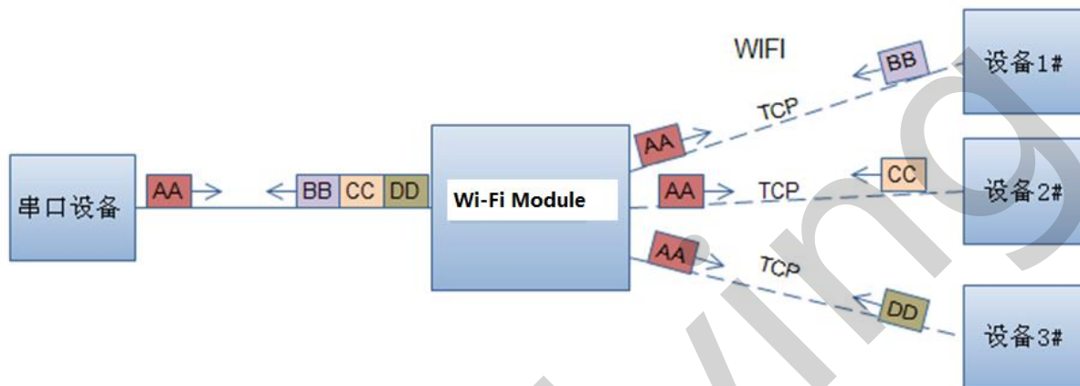
Figure 9. Multi-TCP Link Data Transmission Structure
