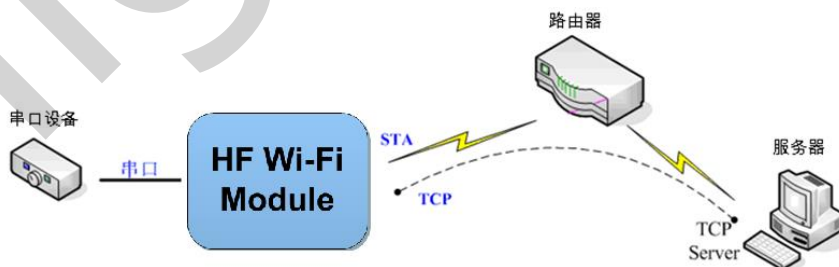
Figure 7. HF-LPB125 STA Network Structure
