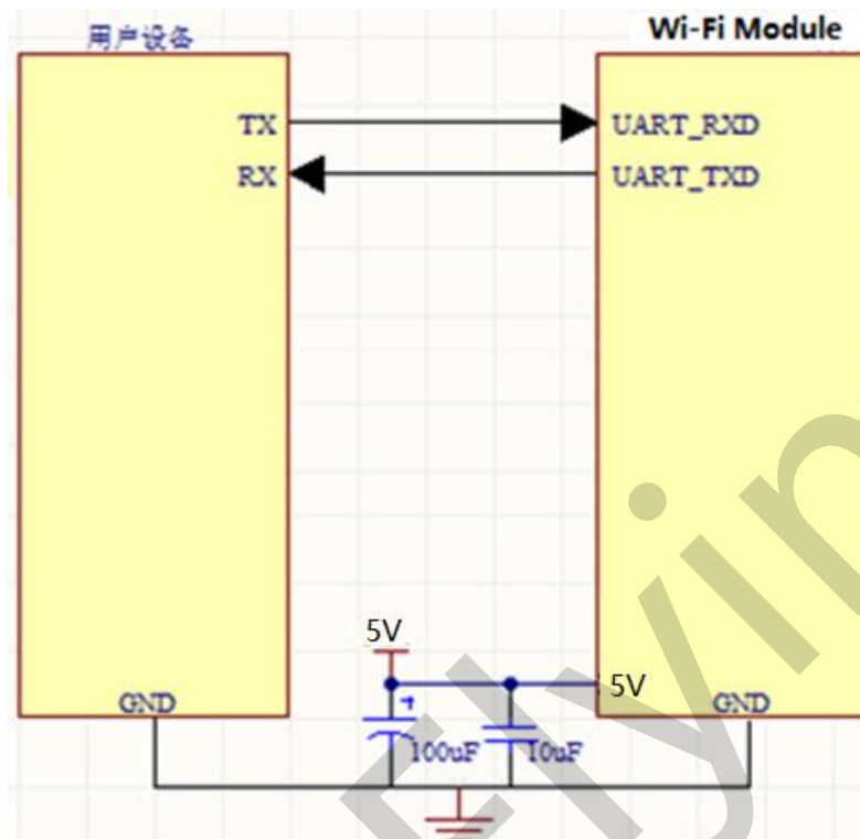
Figure 5. HF-LPB125 Hardware Typical Application
