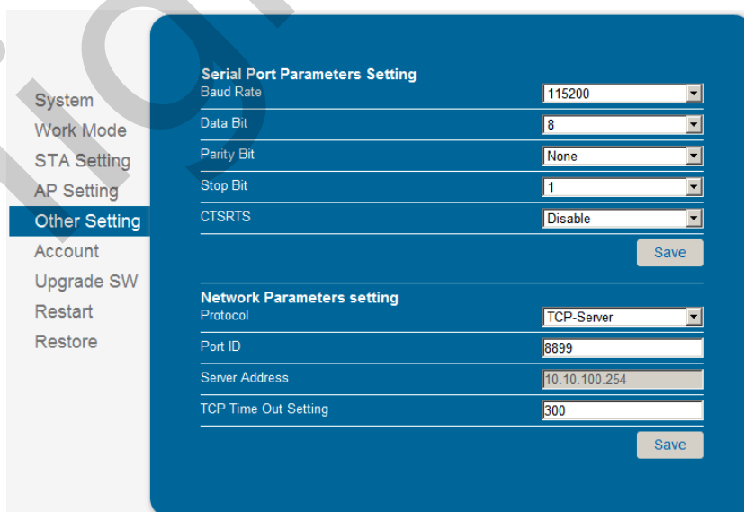
Figure 16. Other Setting Page
