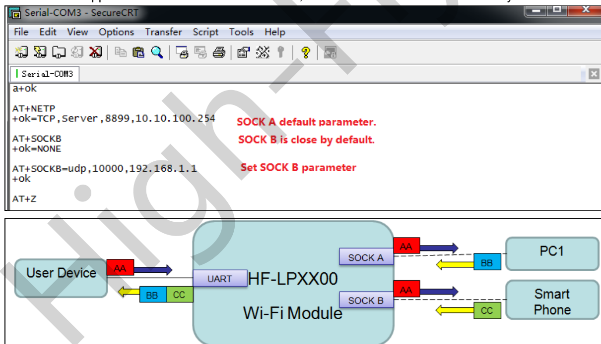
Figure 8. Socket B function demo
