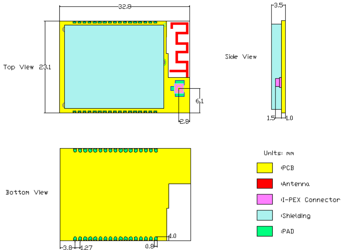
Figure 2. HF-LPB120 机械尺寸
