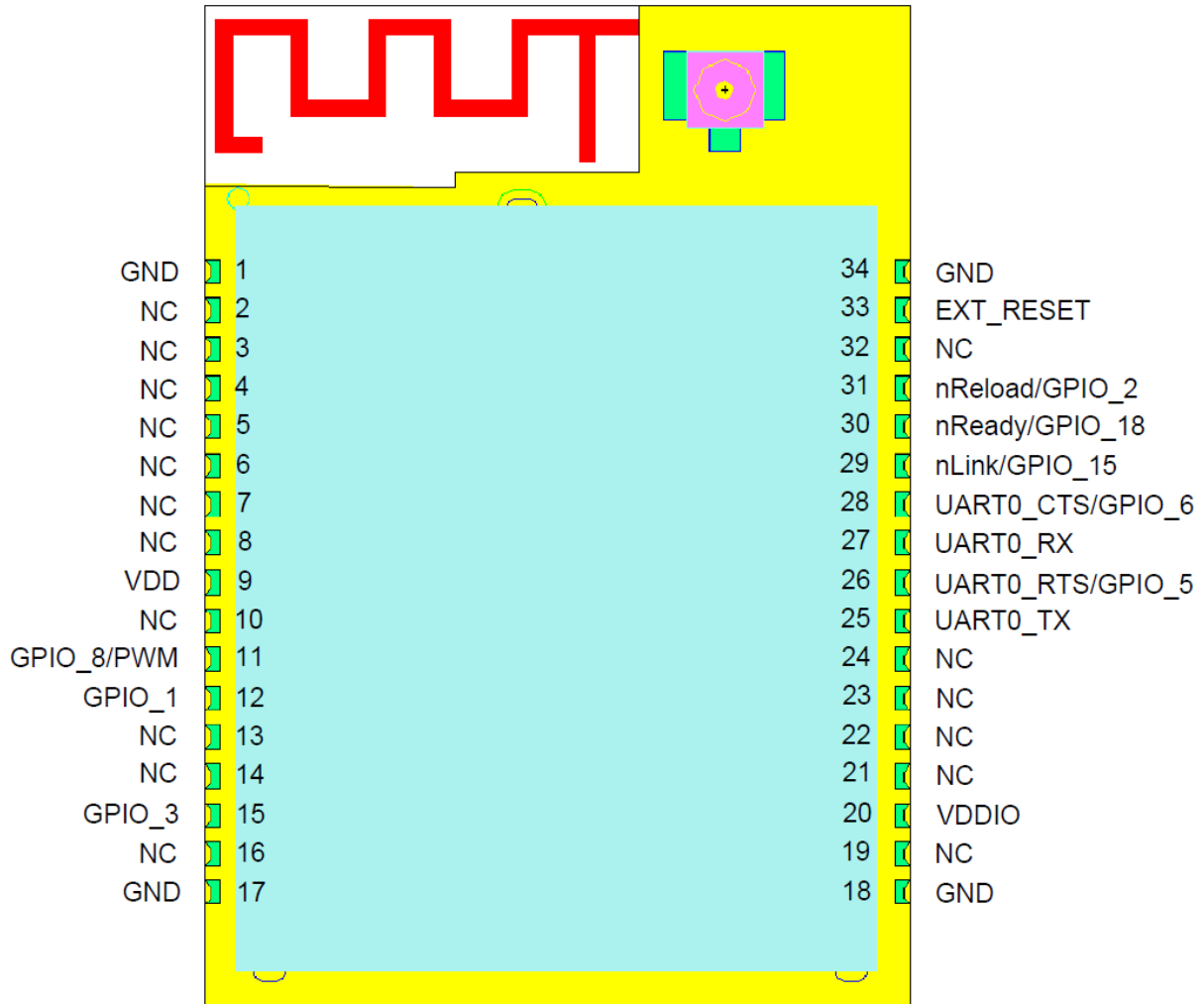
Figure 1. HF-LPB120 管脚定义
