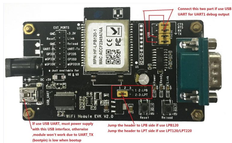
Figure 4. LPB120/LPT120/LPT220 开发板
