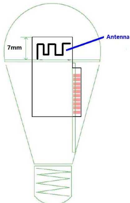
Figure 6. HF-BL300 模块 LED 灯推荐布局
