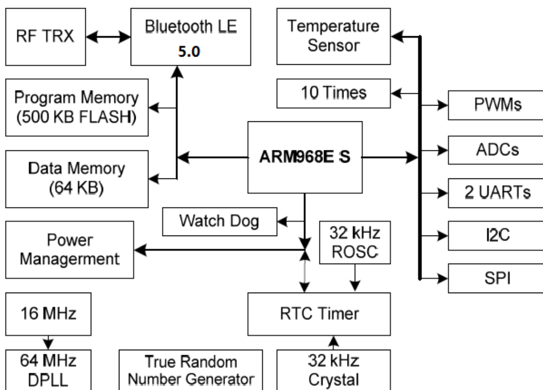
Figure 1. HF-BL300 SOC 芯片架构
