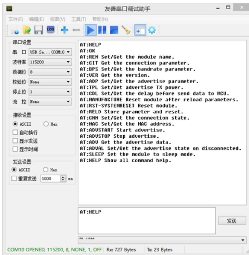
Figure 10. "AT:HELP"列出所有指令示意图
