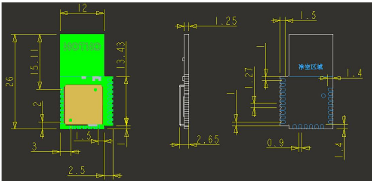
Figure 4. HF-BL300 机械尺寸
