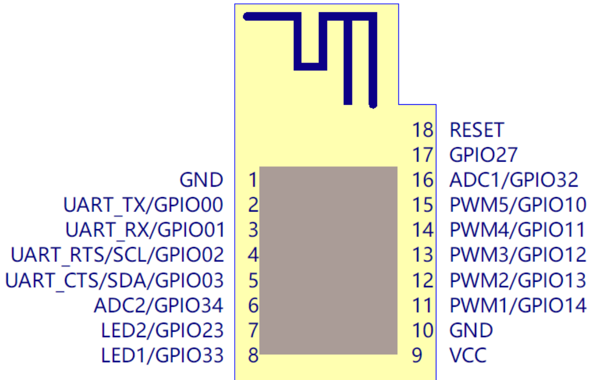
Figure 3. HF-BL300 管脚定义
