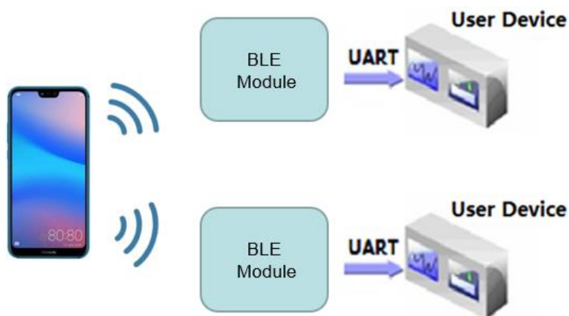
Figure 7. Basic HF-BL300 wireless network structure
