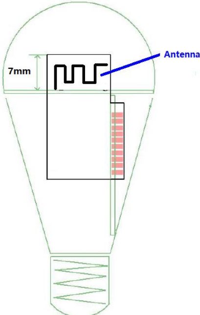
Figure 6. HF-BL300 Module Bulb Reference Placement
