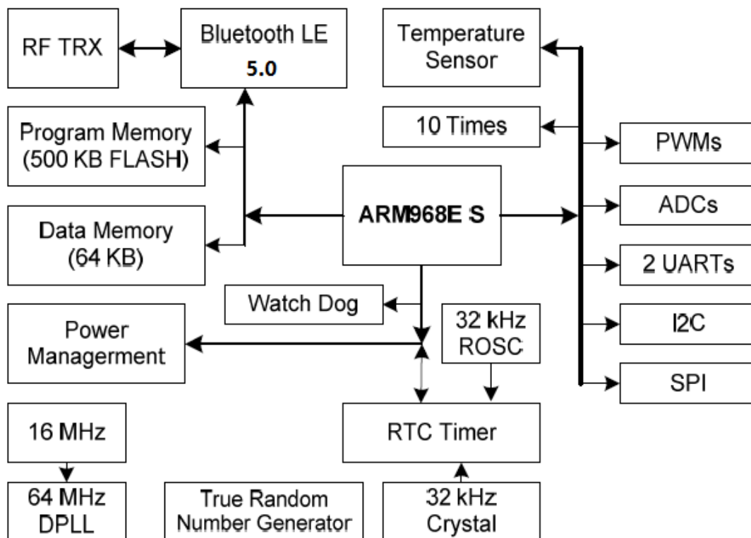
Figure 1. HF-BL300 SOC Block Diagram
