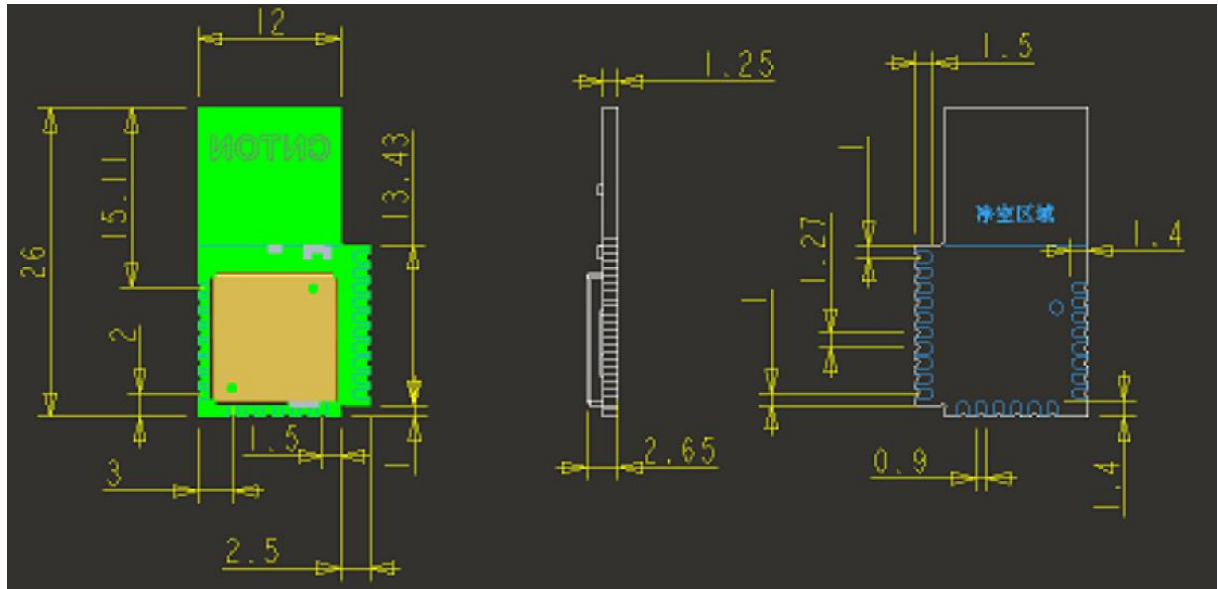
Figure 4. HF-BL300 Mechanical size
