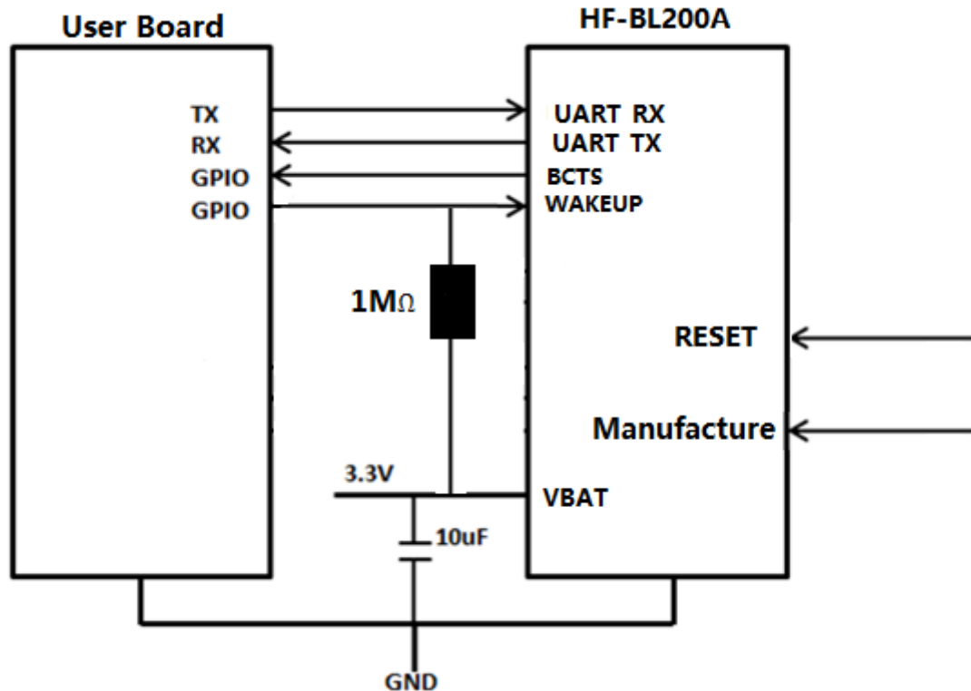
Figure 12. UART Transparent Transmit Typical Application
