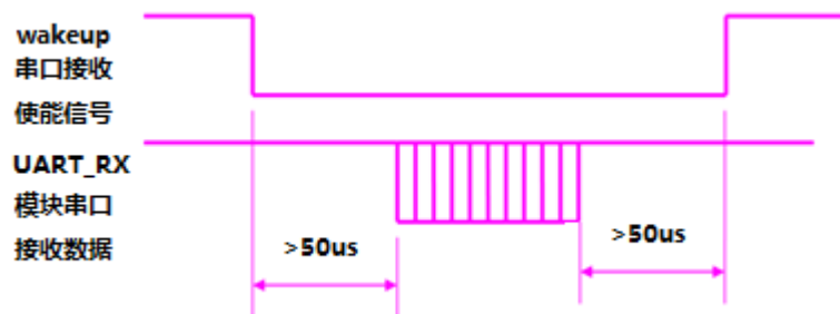
Figure 8. Module UART Receive Enable Signal Map
