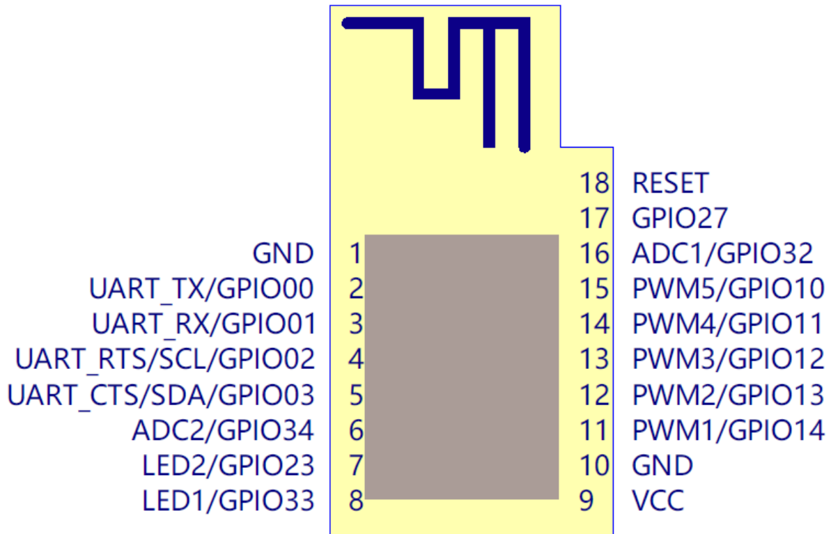
Figure 3. HF-BL300 Pin Definition
