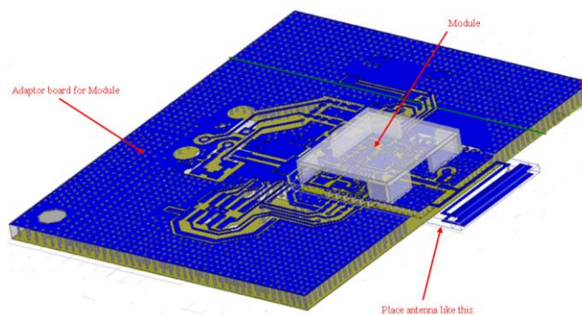
Figure 5. HF-BL300 Module Reference Placement
